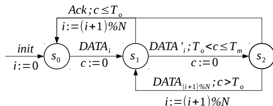
Fig. 1: Monitor State Machine for 802.11 Transmitter.
